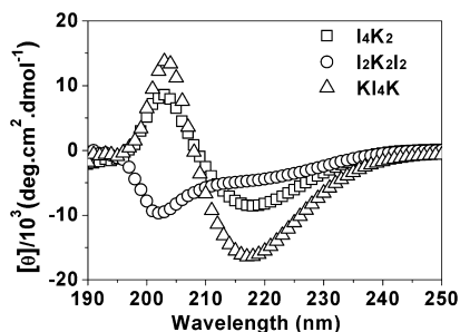
Figure 1. CD spectra of 16 mM I_4K_2 , I_2K_2I_2 , and KI_4K in H_2O at pH 3.0. Prior to CD characterization, the peptide solutions were incubated for 12 days at room temperature. The solvent spectra were subtracted as the background.
