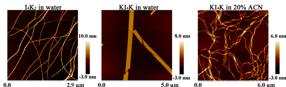
Figure 4. Tapping-mode AFM height images of the assemblies formed by 16 mM I 4 K 2 in water and 16 mM KI 4 K in water and the mixture of acetonitrile (ACN) and water (1:4, v/v). All samples were prepared by directly dissolving the peptide in the solvents, and then the solution pH was slightly adjusted to 3.0. The peptide solutions were incubated for about 12 days at room temperature before AFM characterization.
