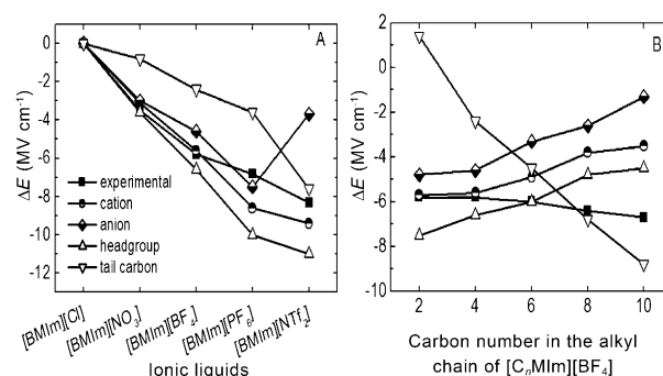
Figure 4. Relative electric fields of A) [BMIm][X] ILs and B) [C n MIm][BF 4 ] ILs determined by the VSE Experiments and the MD simulations for the cations, anions, cationic headgroups, and cationic tail carbon atoms, respectively.
