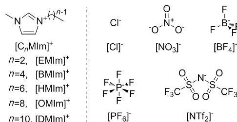
Figure 1. Structures and abbreviations of the cations and the anions being investigated.
