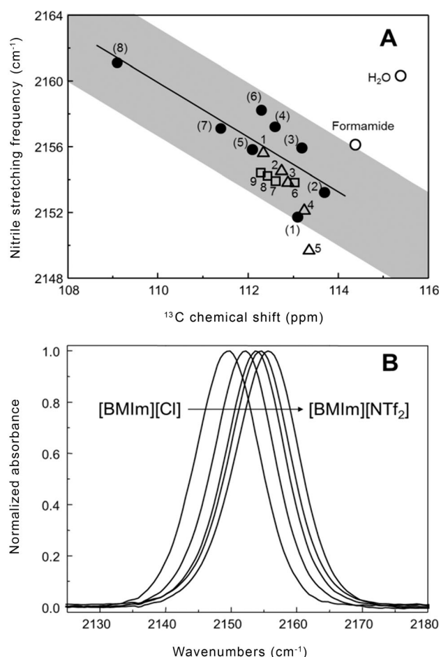
Figure 2. A) Nitrile stretching frequencies \nu_{\text{C}\equiv\text{N}} versus ^{13}\text{C} chemical shifts \delta(^{13}\text{C}) in ILs and molecular solvents (data of molecular solvents were from ref. [14]). Molecular solvents (●): (1) DMSO, (2) DMF, (3) acetone, (4) \text{CD}_2\text{Cl}_2 , (5) THF, (6) \text{CDCl}_3 , (7) toluene, (8) cyclohexane. [BMIm][X] ILs (Δ): 1-[BMIm][NTf 2 ], 2-[BMIm][PF 6 ], 3-[BMIm][BF 4 ], 4-[BMIm][NO 3 ], 5-[BMIm][Cl]. [C n MIm][BF 4 ] ILs (□): 6-[EMIm][BF 4 ], 7-[HMIm][BF 4 ], 8-[OMIm][BF 4 ], 9-[DMIm][BF 4 ]. The black line indicates the best fit for the \nu_{\text{C}\equiv\text{N}} versus ^{13}\text{C} NMR data of molecular solvents excluding H-bonding solvents. [14] B) Normalized IR absorption spectra of \nu_{\text{C}\equiv\text{N}} in [BMIm]-based ILs (from left to right: [Cl], [NO 3 ], [BF 4 ], [PF 6 ], and [NTf 2 ], respectively).
